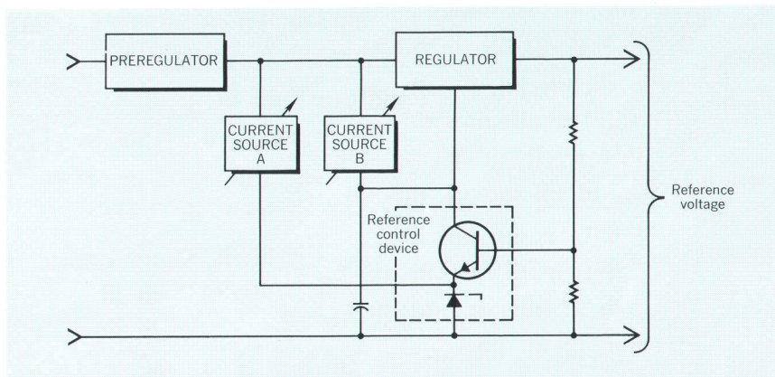
Fig. 5. The 11-volt precision reference supply is a combination of a Zener reference diode and a control transistor. The control transistor generates the correction signal to keep the output at its specified level.
