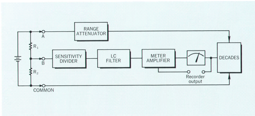
Fig. 4. In the ratiometer mode of operation, the hp-Model 3420A/B acts as a modified Wheatstone bridge to make voltage and resistance divider measurements. The range attenuator and decade divider make up one side of the bridge and the meter amplifier acts as the null detector. The connections from A to COMMON and B to COMMON are the other side of the bridge.
